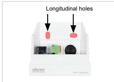
Fig. 6 The device is installed with two screws. Break off the two longitudinal holes in the housing.
