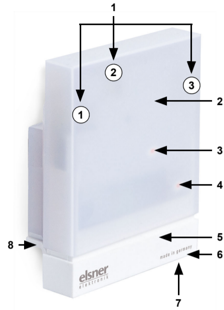
Fig. 4 1 Position of the brightness sensors 1-3. With alignment of the device to the south Sensor 1 = West Sensor 2 = South Sensor 3 = East 2 Semi-transparent cover Vari KNX TH-D GPS: GPS receiver and pressure sensor below. Vari KNX TH-D: pressure sensor below. 3 Position of the Signal LED (under the cover). LED is freely controlled via two objects
