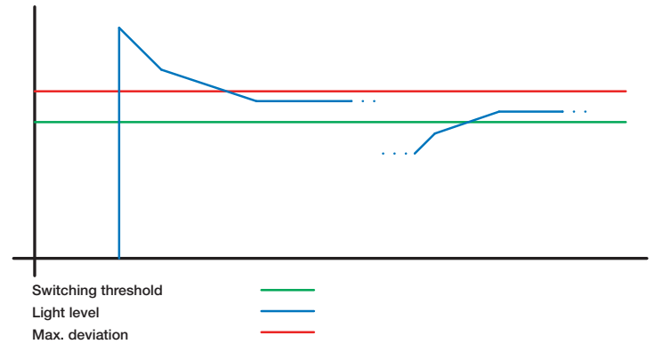
Figure 3: Constant-lighting control range corrected
