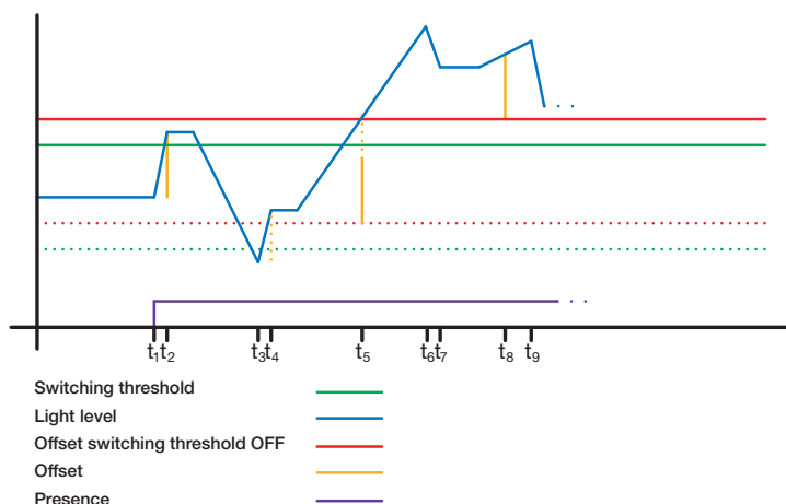
Figure 2: Example 2, switching OFF on the basis of light level
