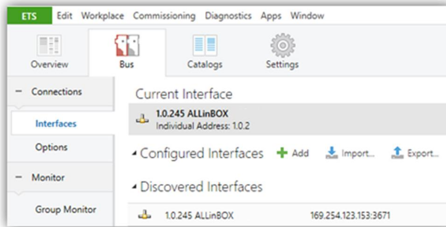
Figure 4. Selection of ALLinBOX in the Bus Connections tab in ETS.
