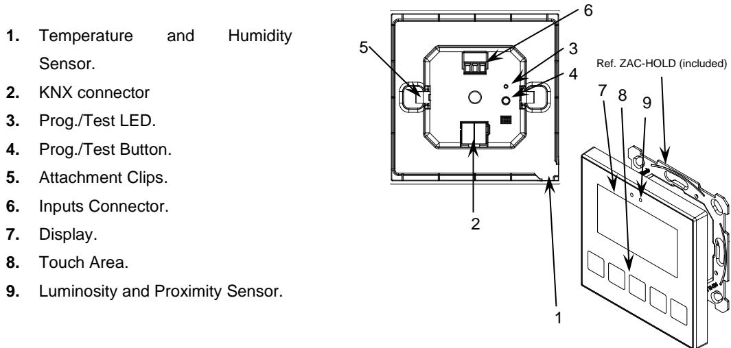
Figure 1. Schematic diagram.
