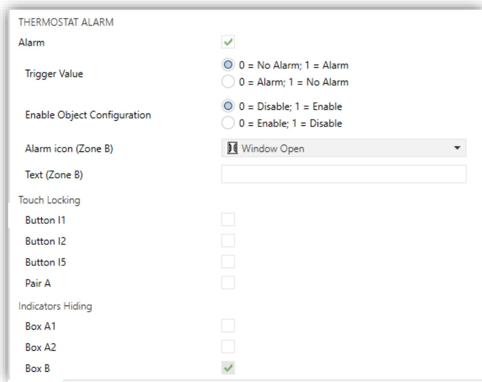
Figure 47. Display – Configuration (Thermostat Page) - Alarm
