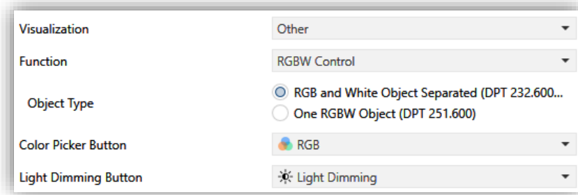
Figure 95. RGBW Control
