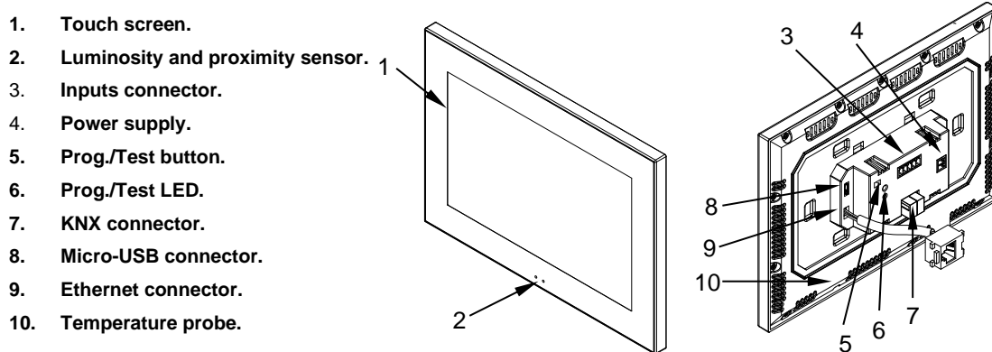
Figure 1 Schematic diagram.
