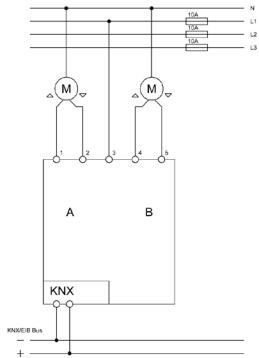
Anschluß JAL-0410.02 - Exemplary circuit diagram JAL-0410.02
