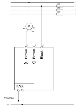
Anschluß JAL-01UP.02 - Exemplary circuit diagram JAL-01UP.02
