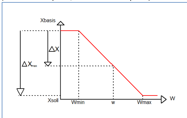
Figure 32: Example – Reference control/decrease
