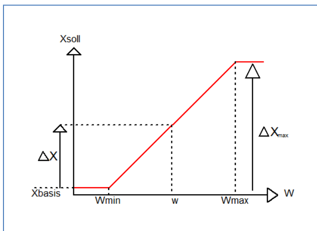
Figure 33: Example – Reference control/increase
