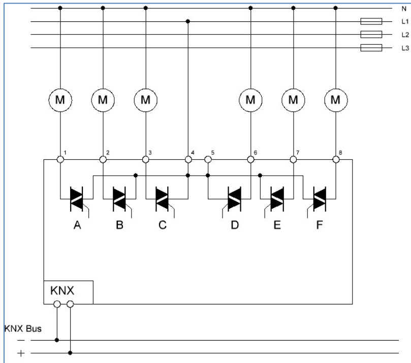
Figure 1: Exemplary circuit diagram – AKH-0600.03
