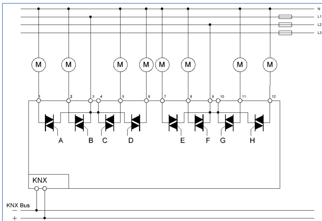
Figure 2: Exemplary circuit diagram – AKH-0800.03
