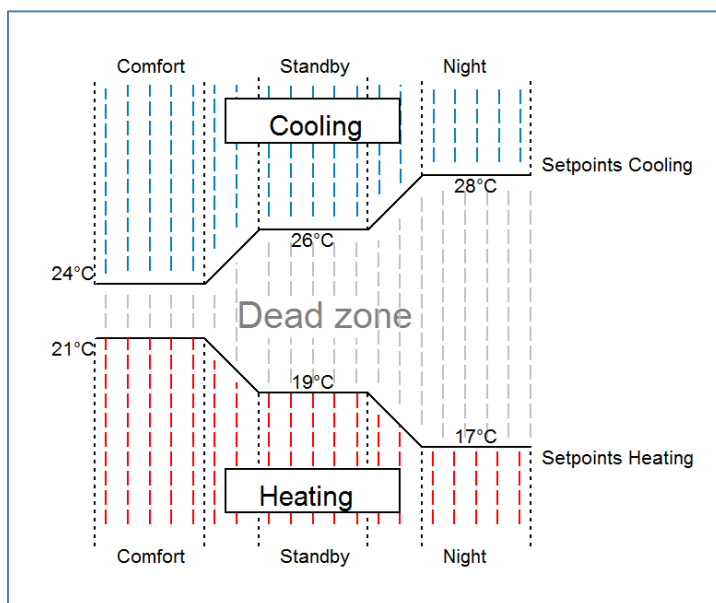
Figure 28: Example – Dead zone and corresponding setpoints
