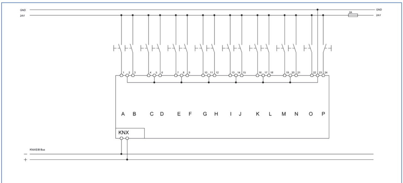
Figure 3: Exemplary circuit diagram BE16024.01 standard configuration for 24V AC/DC input voltage
