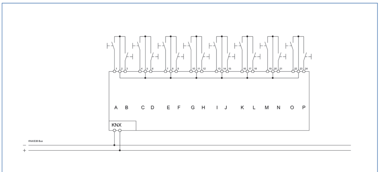
Figure 1: Exemplary circuit diagram BE16000.01 standard configuration for floating contacts
