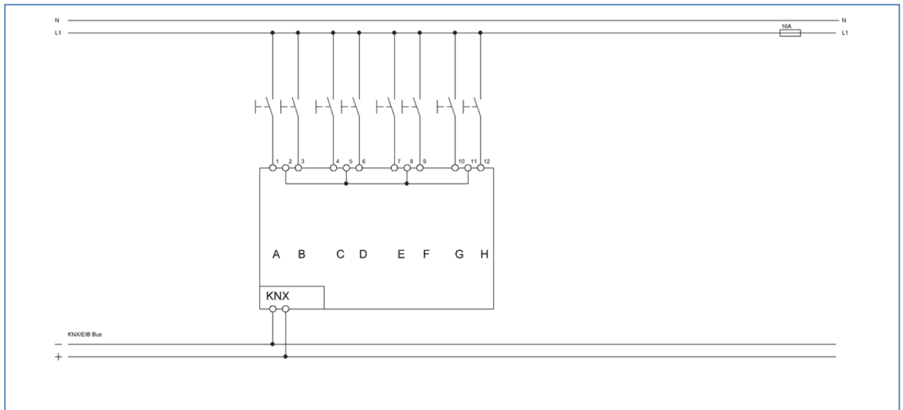
Figure 6: Exemplary circuit diagram BE08230.01 standard configuration for 230V AC input voltage
