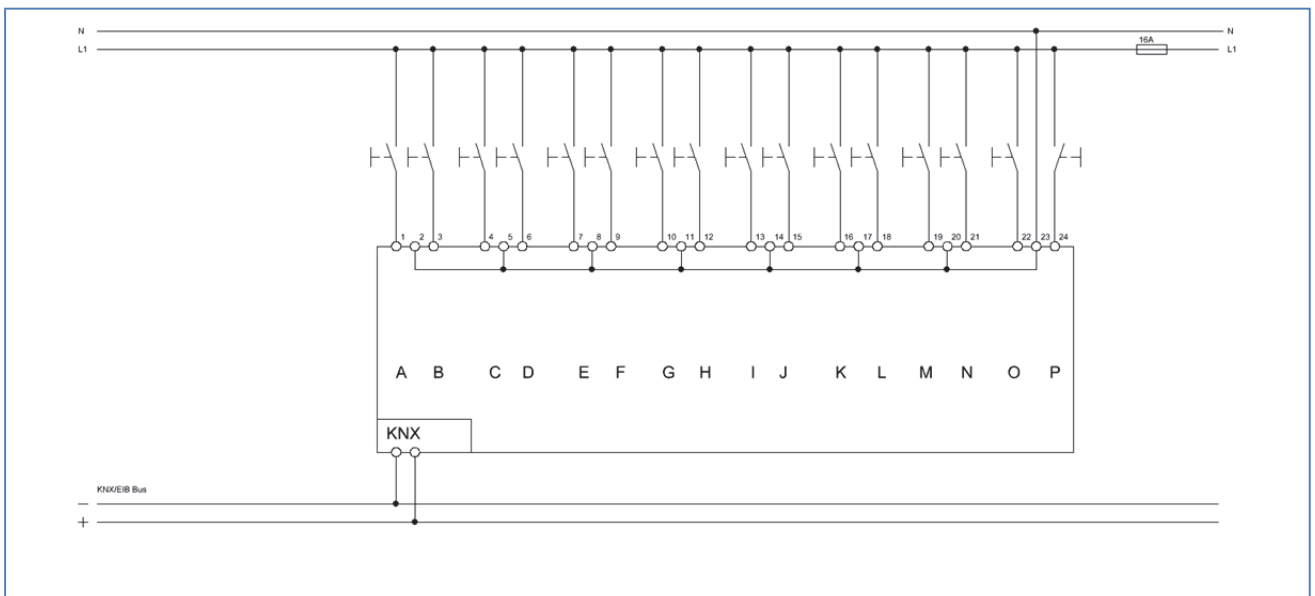
Figure 5: Exemplary circuit diagram BE16230.01 standard configuration for 230V AC input voltage
