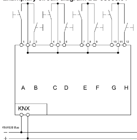
Exemplary circuit diagram BE-08230.01
