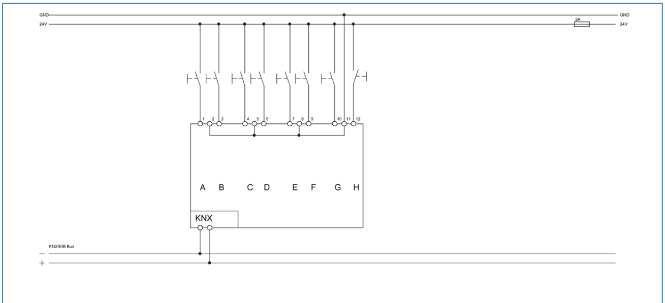
Figure 4: Exemplary circuit diagram BE08024.01 standard configuration for 24V AC/DC input voltage
