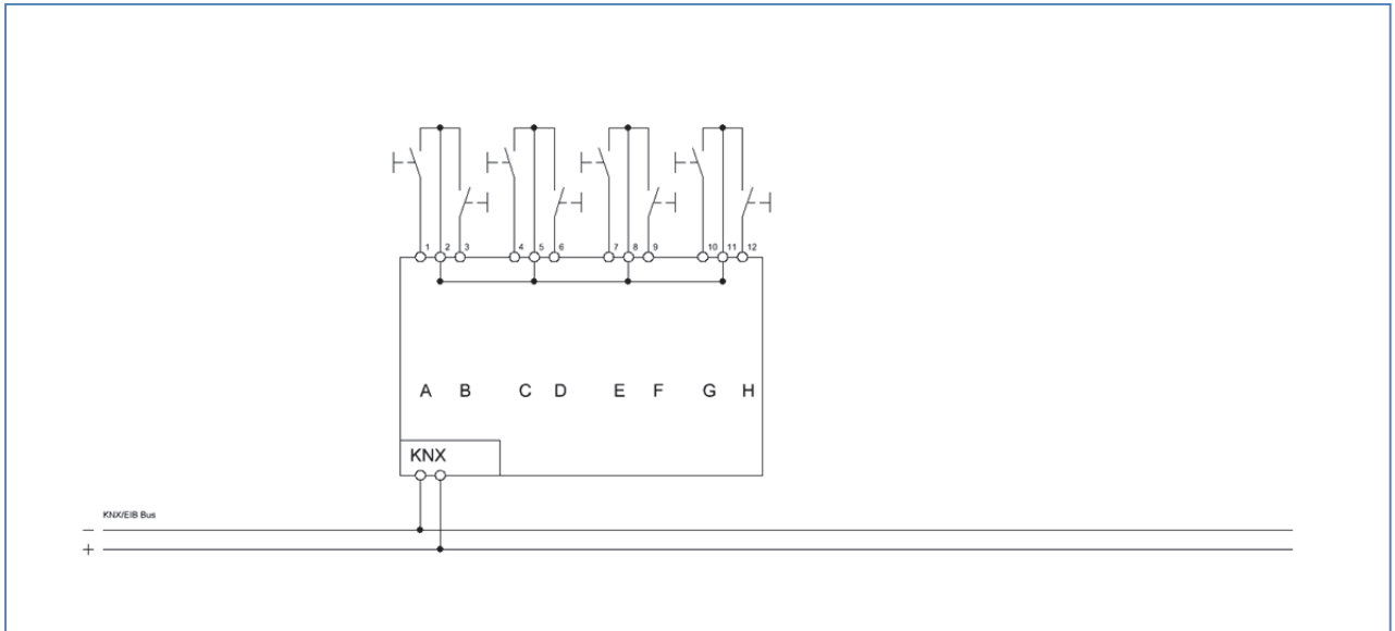
Figure 2: Exemplary circuit diagram BE08000.01 standard configuration for floating contacts
