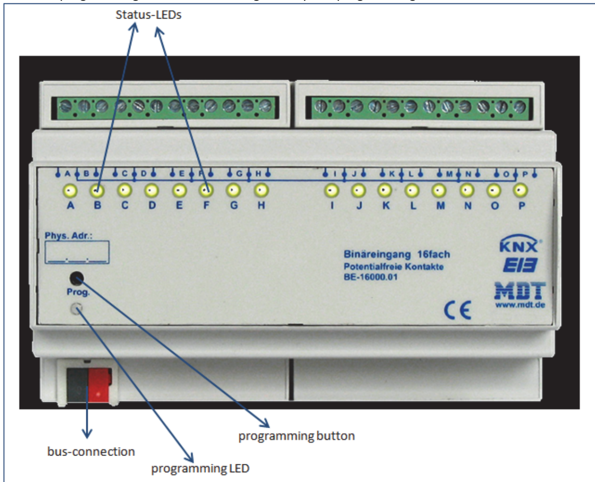
Figure 7: Overview hardware module binary input (BE-16000.01 for floating contacts)
