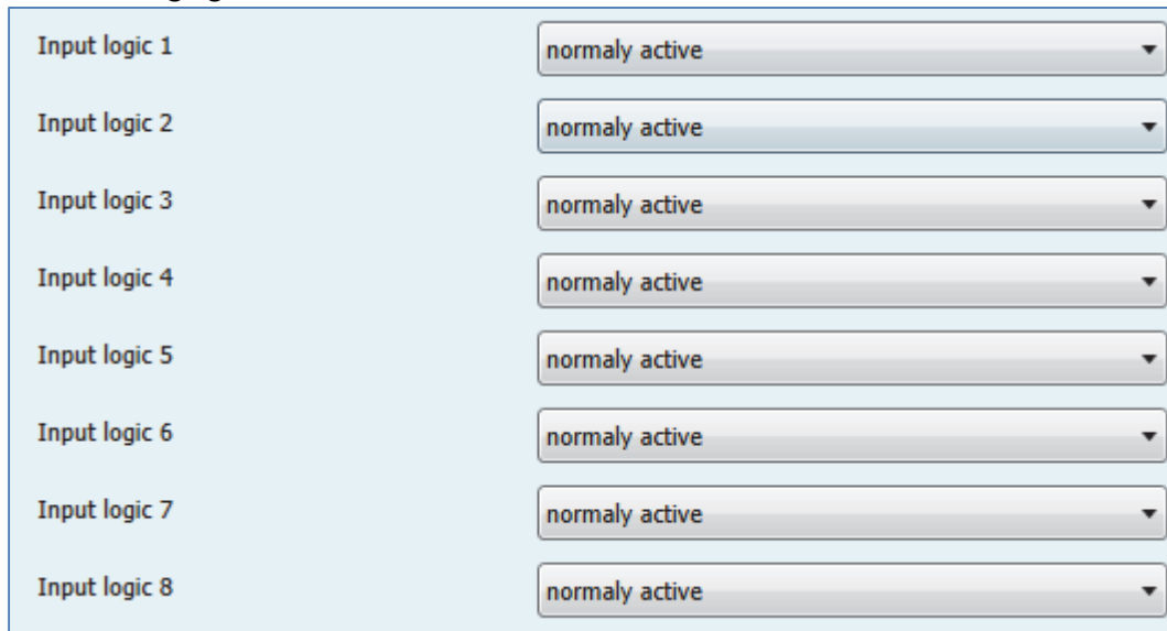
Figure 16: Submenu logic
