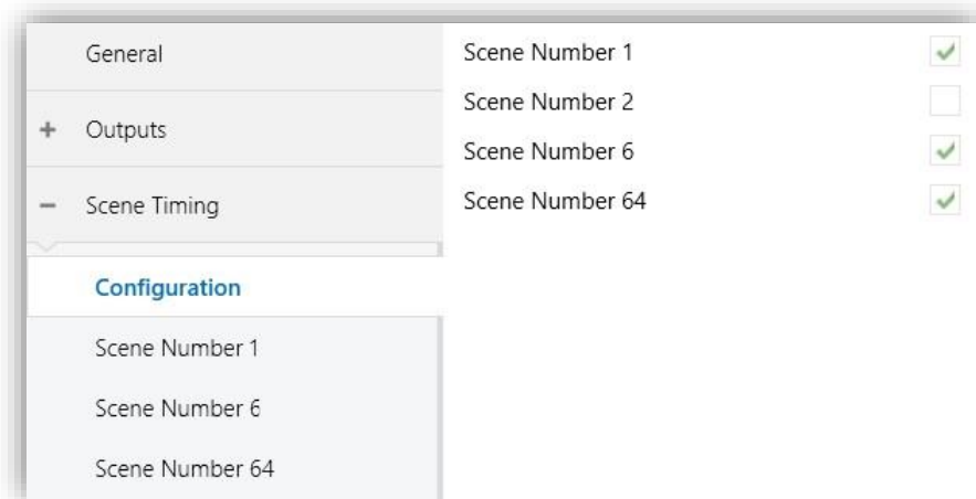
Figure 5. Scene Temporization
