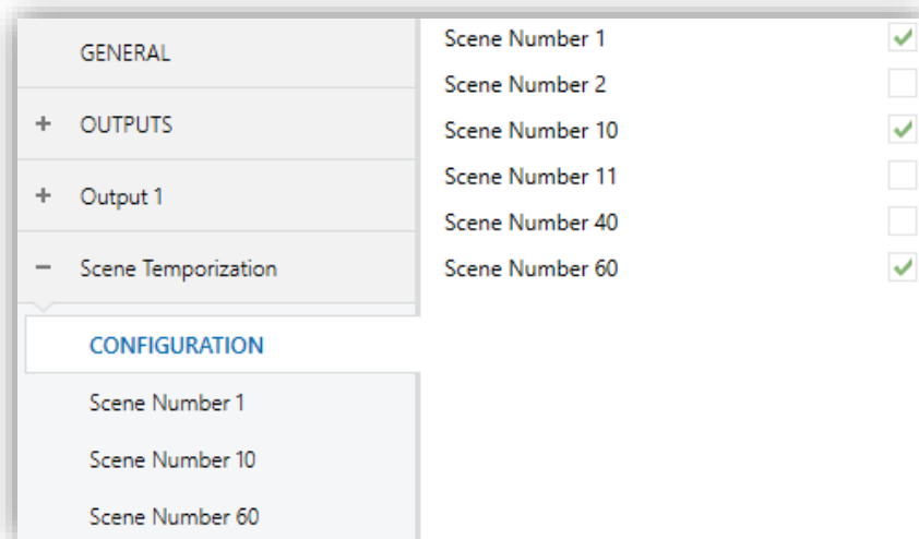
Figure 5. Scene Temporization
